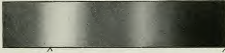
Invisible Ultra-Violet Limit of Visibility Violet Blue Blue-Green Green Yellow-Green Orange Red Deep-Red Limit of Visibility Fig. 107.
